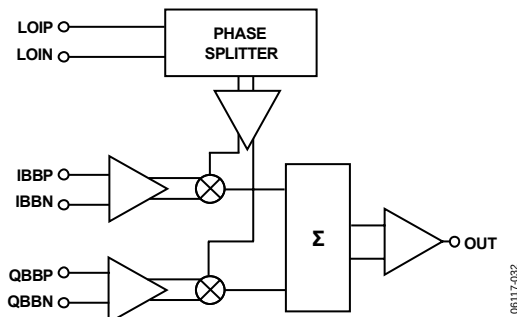
Figure 24. Block Diagram
