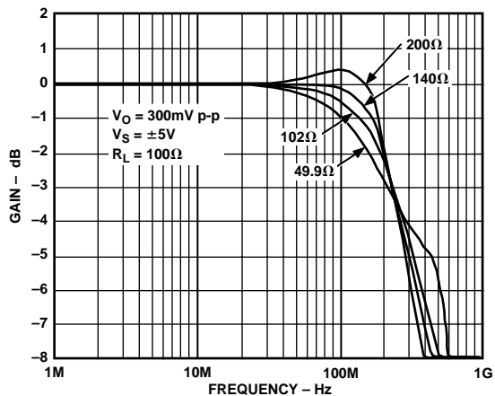
Figure 15. AD8036 Small Signal Frequency Response, G = +1
