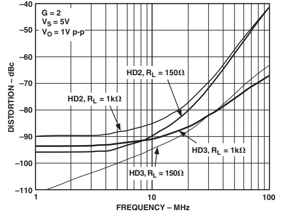
TPC 22. AD8008 Second and Third Harmonic Distortion vs. Frequency and R_L
