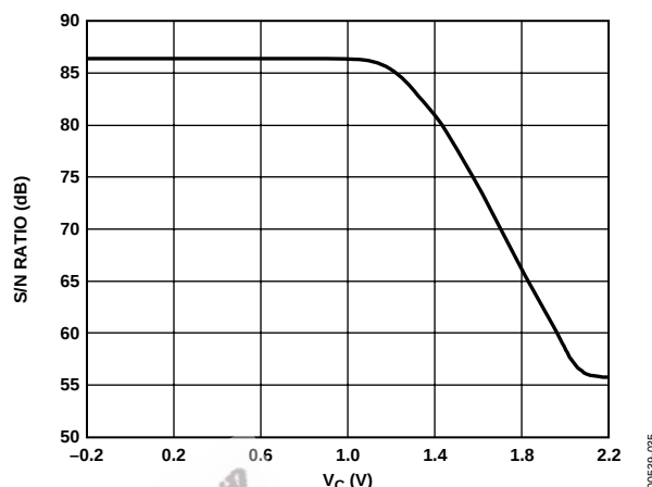
Figure 35. SNR vs. Control Voltage–Sequential Control (1 MHz Bandwidth)
