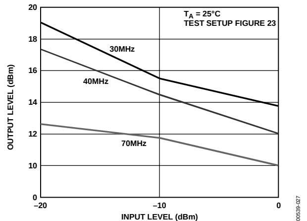
Figure 27. Third Order Intercept -10 dB/+30 dB Mode, Gain = +10 dB
