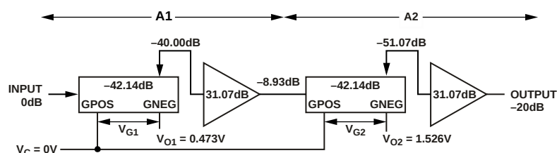
Figure 36. AD603 Gain Control Input Calculations for Sequential Control Operation V_C = 0 V
