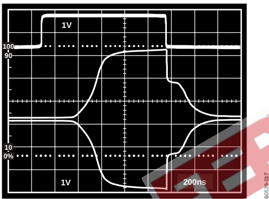
Figure 17. Gain Control Channel Response Time
