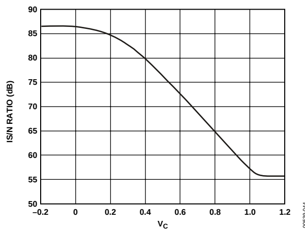
Figure 44. ISNR for Cascaded Stages—Parallel Control
