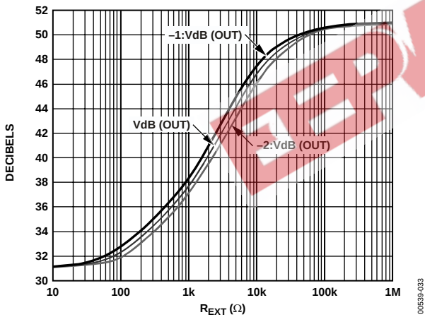
Figure 33. Gain vs. R_{EXT} , Showing Worst-Case Limits Assuming Internal Resistors have a Maximum Tolerance of 20%
