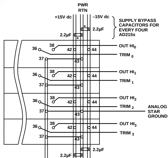
Figure 20a. PCB Layout for Unity Gain
