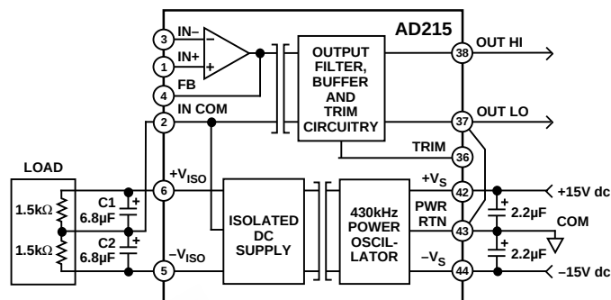
Figure 19. Using the Isolated Power Supplies
