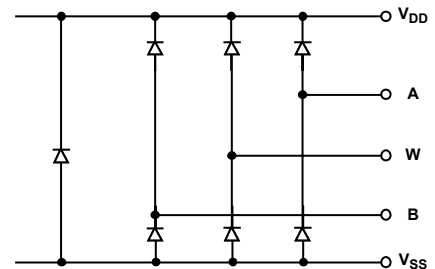
Figure 47. Maximum Terminal Voltages Set by V_{DD} and V_{SS}
