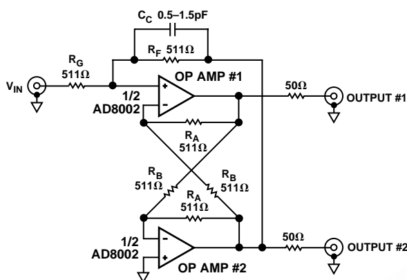
Figure 47. Differential Line Driver
