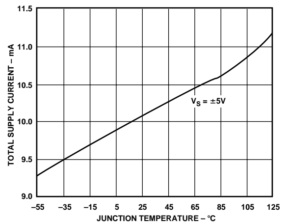
Figure 27. Total Supply Current vs. Temperature
