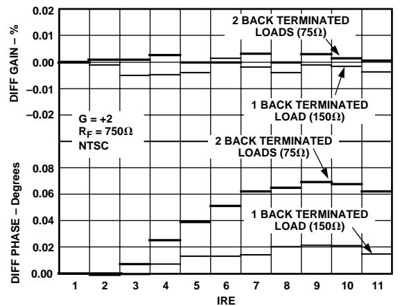
Figure 15. Differential Gain and Differential Phase (per Amplifier)
