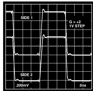
Figure 9. 1 V Step Response, G = +2
