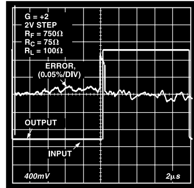
Figure 25. Long-Term Settling Time
