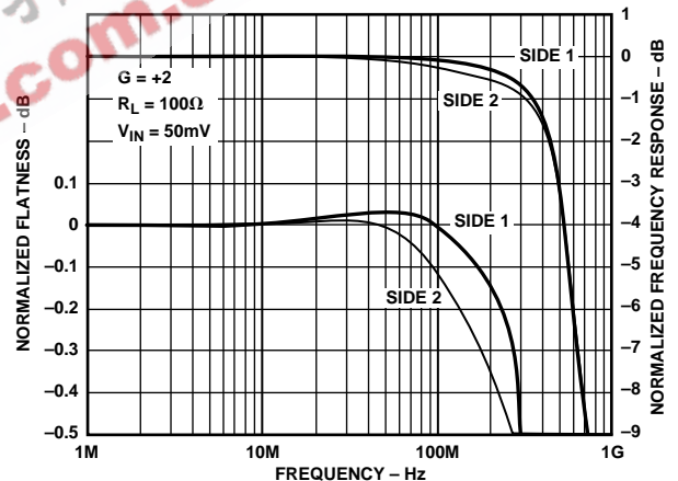
Figure 1. Frequency Response and Flatness, G = +2
