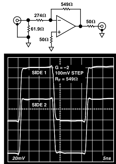
Figure 39. 100 mV Step Response, G = -2
