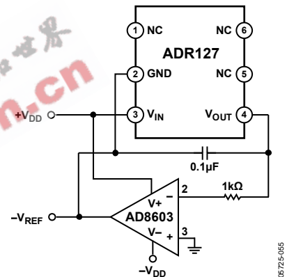
Figure 51. Negative Reference
