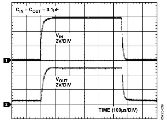
Figure 35. ADR125 Turn-On Response
