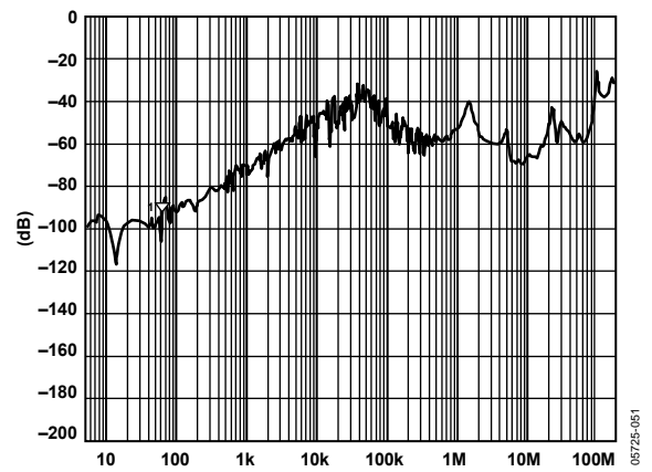
Figure 47. ADR121/ADR125/ADR127 PSRR
