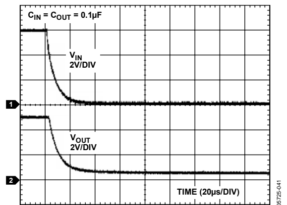
Figure 37. ADR125 Turn-Off Response
