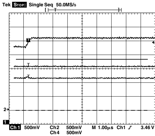
TPC 1. Line Transient Response, Channel 1 and Channel 2
