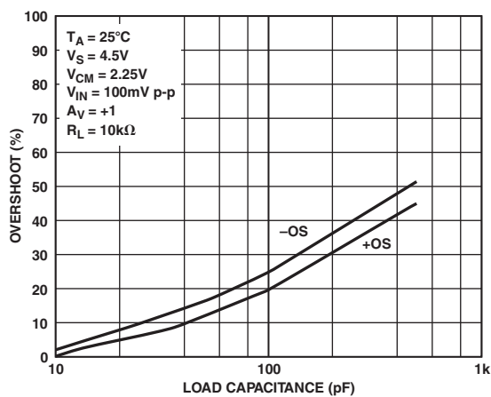
TPC 22. Small Signal Overshoot vs. Load Capacitance, V_S = 4.5 V
