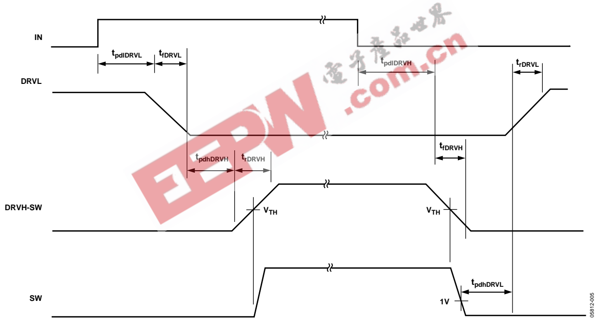
Figure 5. Timing Diagram
