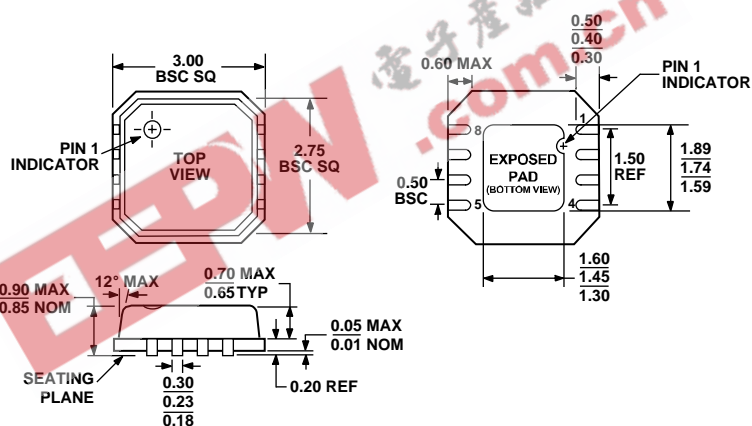
Figure 18. 8-Lead Lead Frame Chip Scale Package [LFCSVP_VD]
