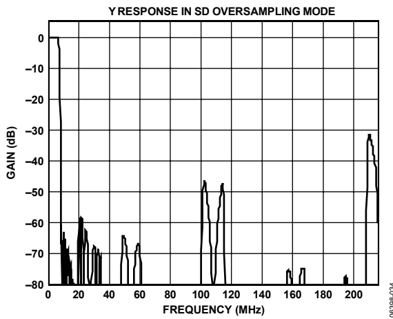
Figure 34. SD, 16× Oversampling, Y Filter Response
