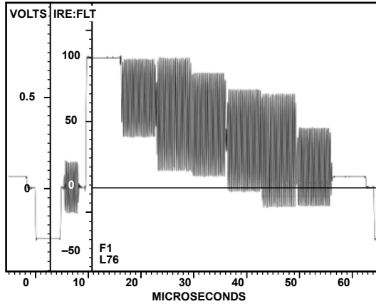
APL = 44.5% 525 LINE NTSC SLOW CLAMP TO 0.00V AT 6.72µs PRECISION MODE OFF SYNCHRONOUS SYNC = A FRAMES SELECTED 1, 2
