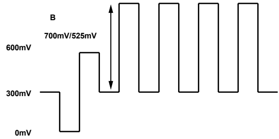
Figure 127. HD RGB Output Levels—RGB Sync Enabled
