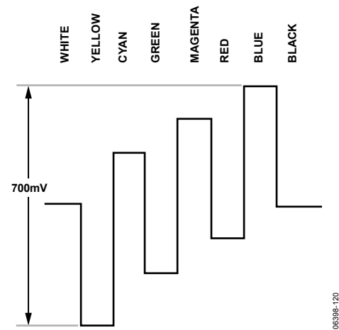
Figure 119. Pb Levels—PAL
