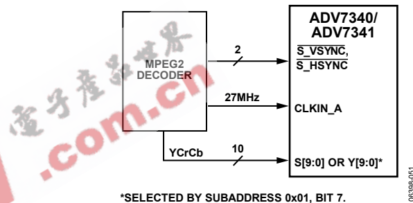
Figure 51. SD Only Example Application
