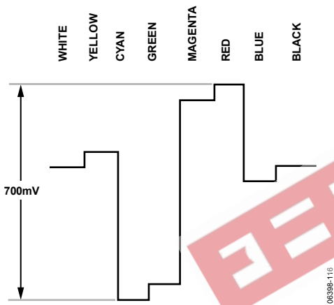
Figure 115. Pr Levels—NTSC
