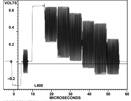
NOISE REDUCTION: 0.00dB APL = 39.1% 625 LINE NTSC NO FILTERING SLOW CLAMP TO 0.00 AT 6.72µs PRECISION MODE OFF SYNCHRONOUS SOUND-IN-SYNC OFF FRAMES SELECTED 1, 2, 3, 4
