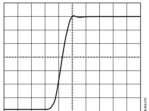
Figure 75. Output Signal from ED/HD Adaptive Filter (Mode A)
