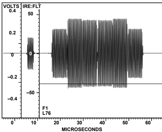
NOISE REDUCTION: 15.05dB APL NEEDS SYNC SOURCE. 525 LINE NTSC NO FILTERING SLOW CLAMP TO 0.00 AT 6.72µs PRECISION MODE OFF SYNCHRONOUS SYNC = B FRAMES SELECTED 1, 2
