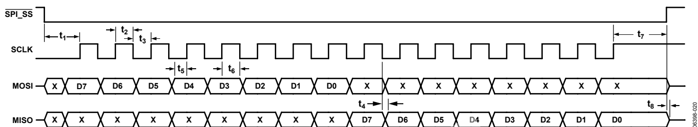
Figure 20. MPU Port Timing Diagram (SPI Mode)
