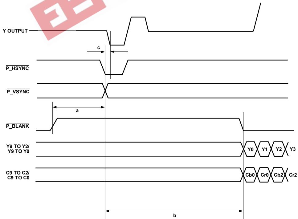
Figure 15. ED-DDR, 8-/10-Bit, 4:2:2 YCrCb (HSYNC/VSYNC) Input Timing Diagram
