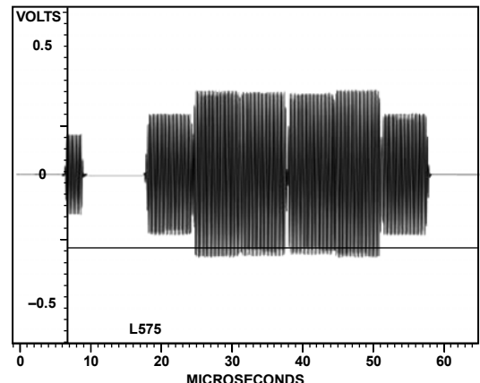
Figure 132. PAL Luma
