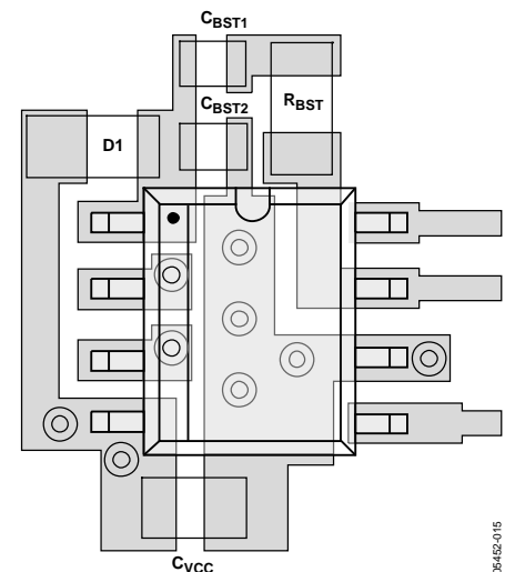
Figure 14. External Component Placement Example
