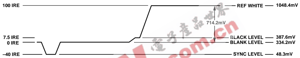
Figure 46. NTSC Luma Video Levels
