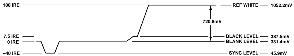
Figure 48. NTSC RGB Video Levels
