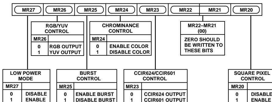
Figure 39. Mode Register 2
