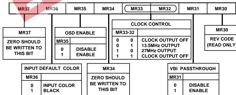
Figure 41. Mode Register 3
