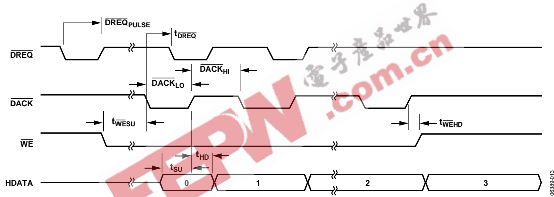
Figure 5. Single Write for DREQ/DACK DMA Mode for Assigned DMA Channel (EDMOD0/EDMOD1 <14:11> Not Programmed to a Value of 0000)
