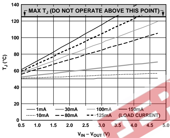
Figure 27. 100 mm 2 of PCB Copper, T A = 50°C
