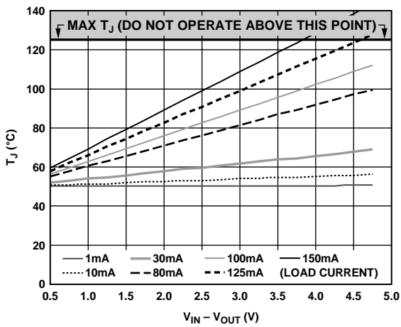
Figure 26. 500 mm 2 of PCB Copper, T A = 50°C
