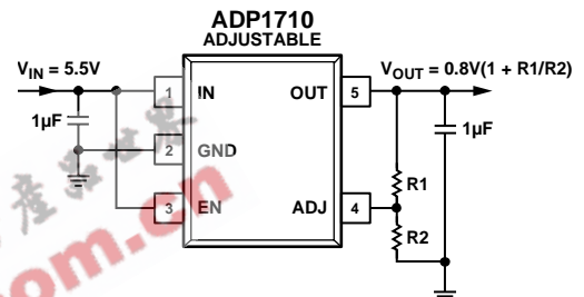
Figure 2. ADP1710 with Adjustable Output Voltage, 0.8 V to 5.0 V
