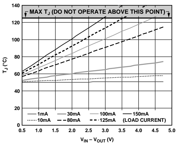
Figure 28. 0 mm 2 of PCB Copper, T A = 50°C
