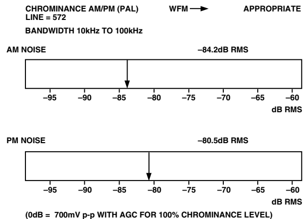
Figure 142. PAL Chrominance AM/PM
