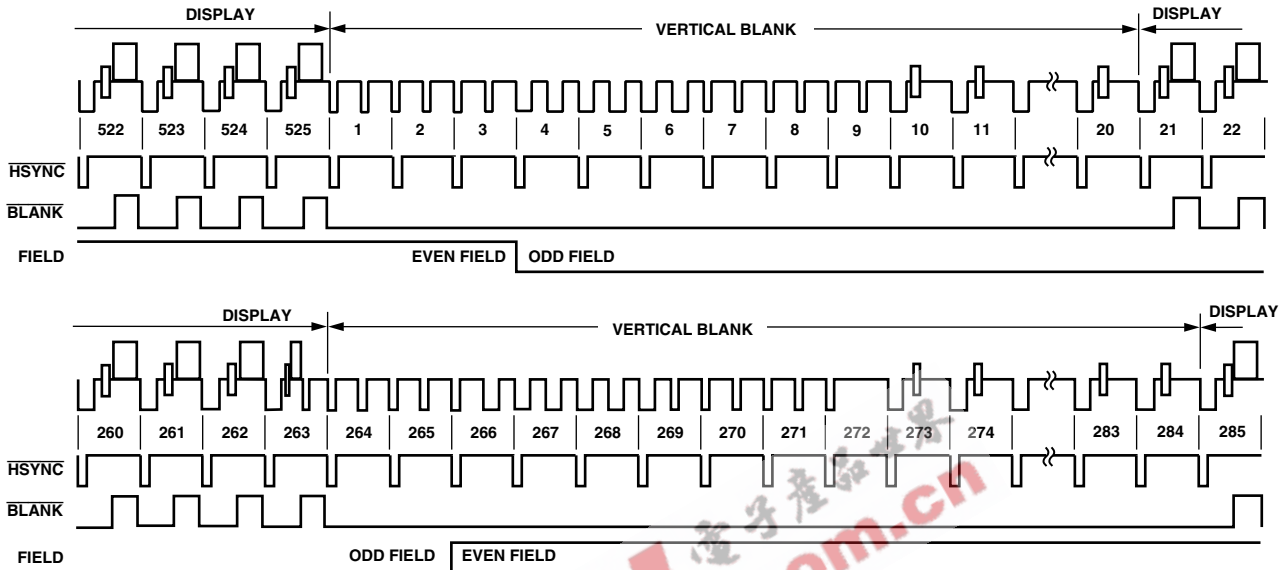
Figure 42. Timing Mode 1, NTSC
