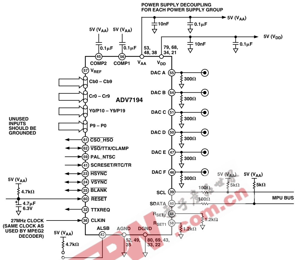
Figure 94. Recommended Analog Circuit Layout
