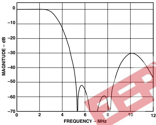
Figure 23. Chroma 3 MHz Low-Pass Filter
