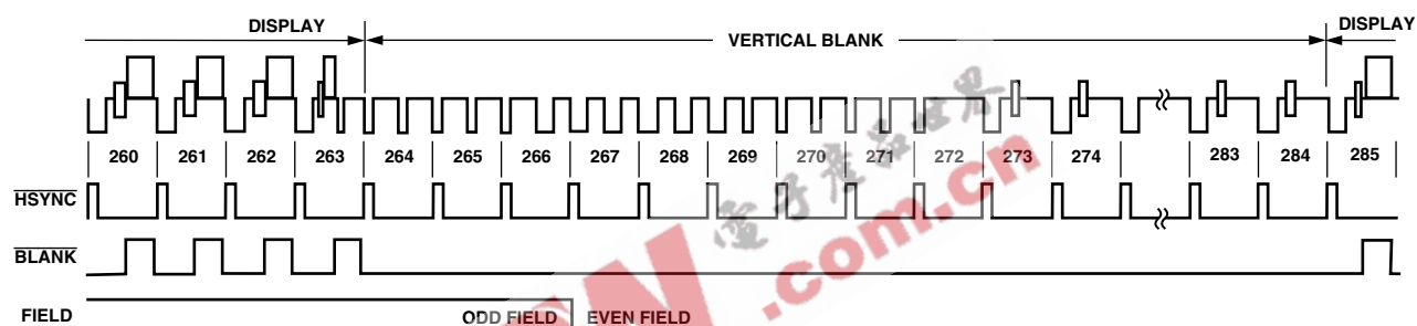
Figure 49. Timing Mode 3, NTSC
