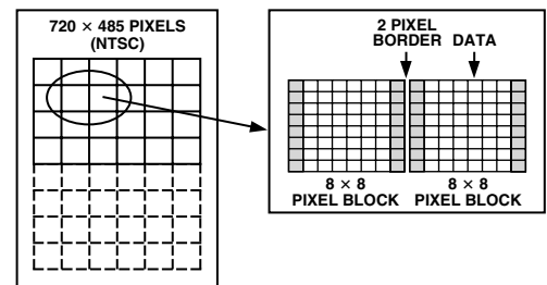
Figure 85. MPEG Block Diagram
