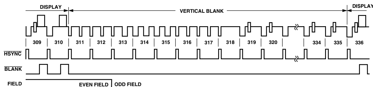
Figure 50. Timing Mode 3, PAL
