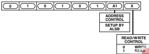
Figure 51. Slave Address
