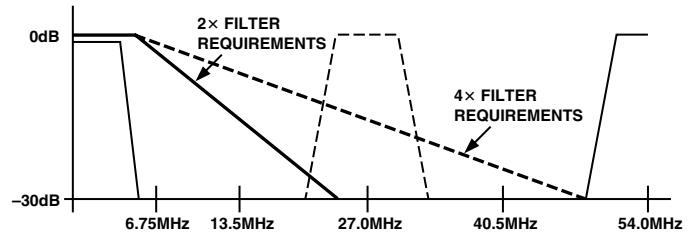
Figure 35b. Output Filter Requirements in 4x Oversampling Mode
