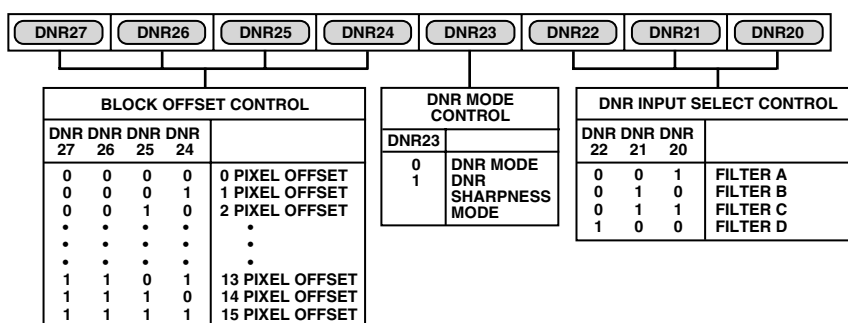
Figure 90. DNR Register 2
