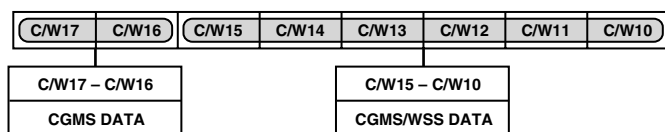
Figure 76. CGMS_WSS Register 1
