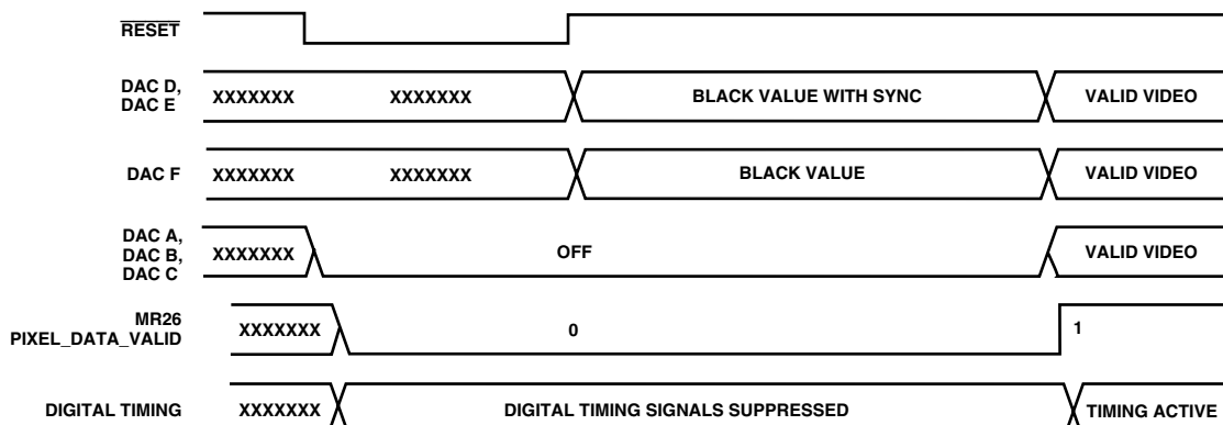
Figure 36. RESET Sequence Timing Diagram
