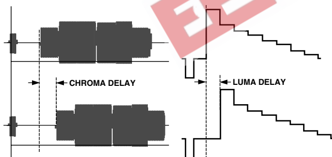
Figure 28. Chroma Delay
