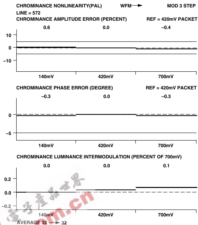
Figure 135. PAL Chrominance Nonlinearity
