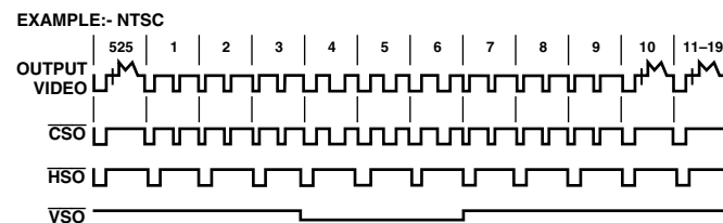
Figure 29. \overline{CSO} , \overline{HSO} , \overline{VSO} Timing Diagram
