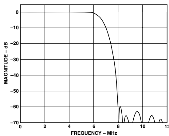
Figure 11. Extended Mode (SSAF) Luma Filter
