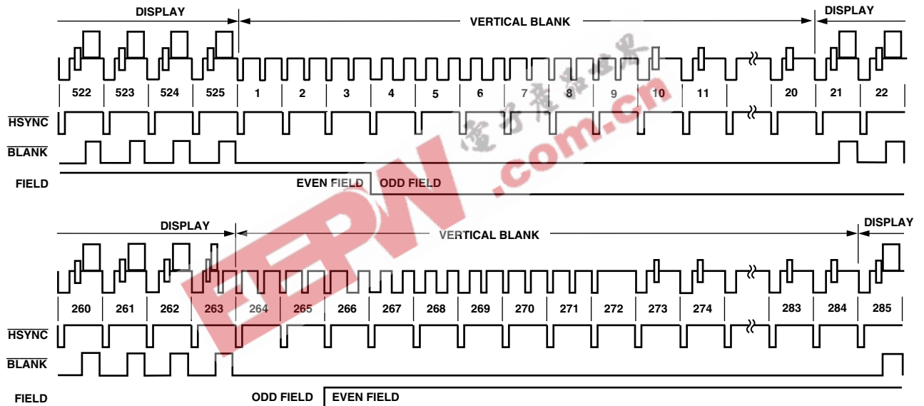
Figure 37. Timing Mode 1, NTSC
