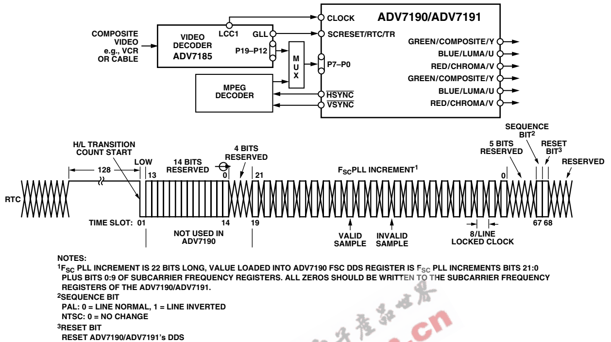
Figure 32. RTC Timing and Connections
