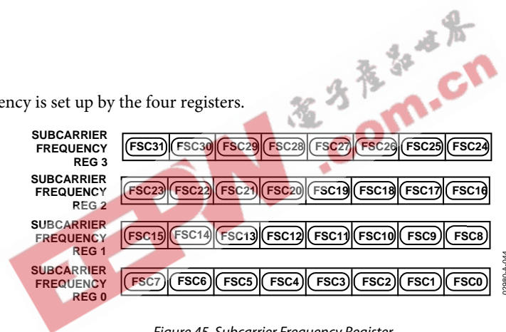
Figure 45. Subcarrier Frequency Register
