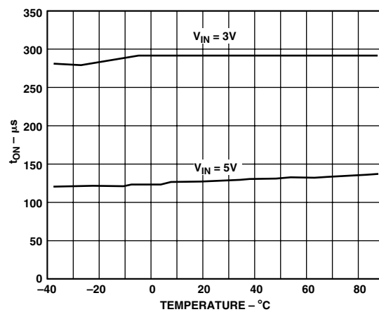
TPC 8. Turn-On Time vs. Temperature
