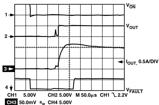
TPC 13. Switch Turn-On Time
