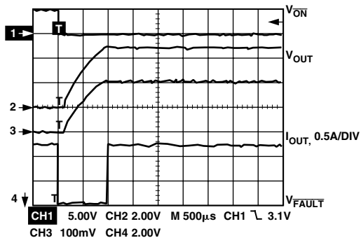
TPC 15. USB Circuit Output Rise Time
