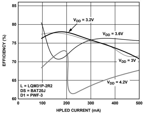
Figure 13. Efficiency P_{LED}/P_{IN} , One High Power White LED
