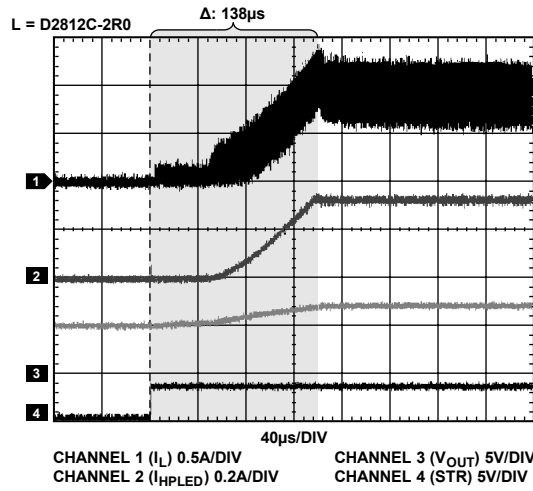
Figure 5. Startup, Two LEDs Flash Mode, LED Current = 335 mA, V_{DD} = 3.2\text{ V}
