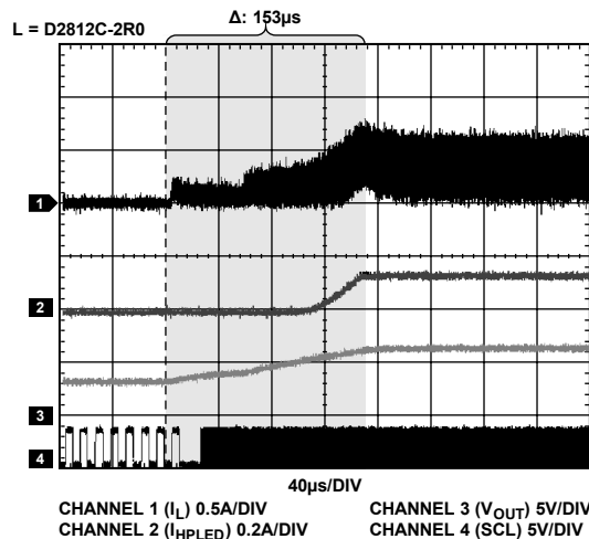
Figure 7. Startup, Two LEDs Torch Mode, LED Current = 130 mA, V_{DD} = 3.2\text{ V}
