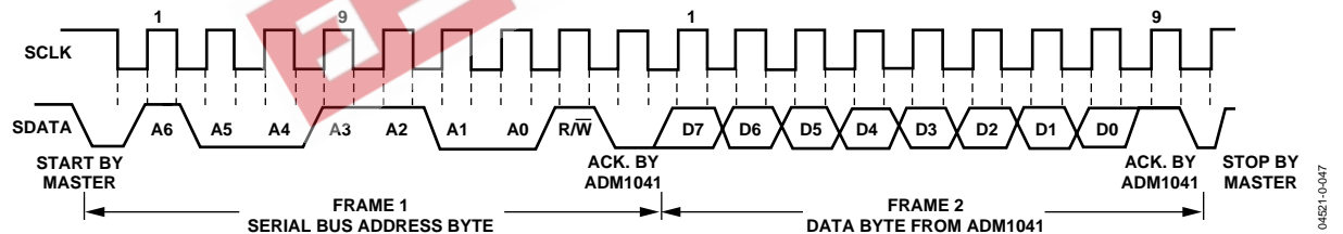
Figure 27. Reading Data from a Previously Selected Register
