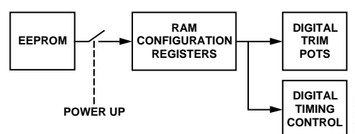
Figure 37. EEPROM Download
