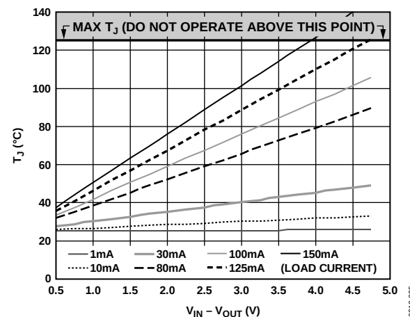
Figure 25. 0 mm 2 of PCB Copper, T_A = 25^\circ\text{C}
