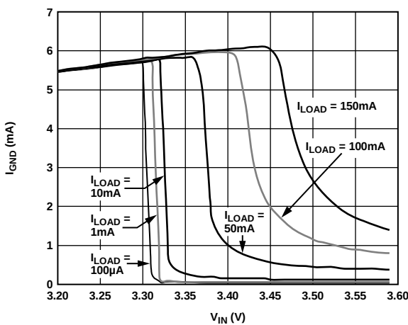
Figure 15. Ground Current vs. Input Voltage (In Dropout)
