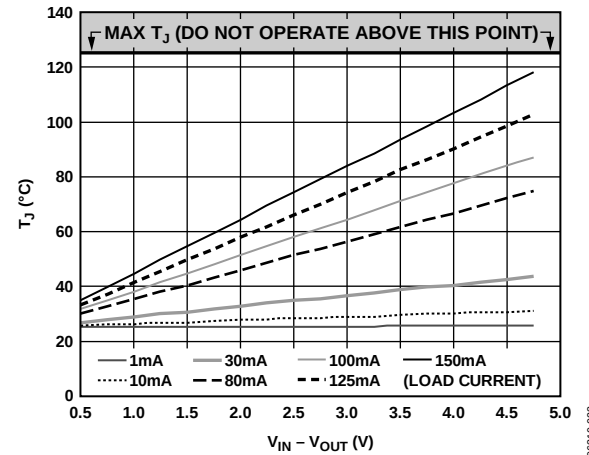
Figure 23. 500 mm 2 of PCB Copper, T_A = 25^\circ\text{C}
