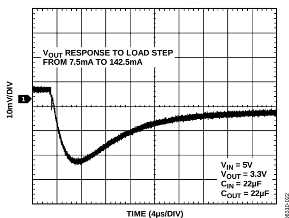
Figure 22. Output Transient Response, C_{OUT} = 22\text{ }\mu\text{F}
