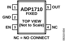
Figure 4. 5-Lead TSOT (UJ-Suffix)
