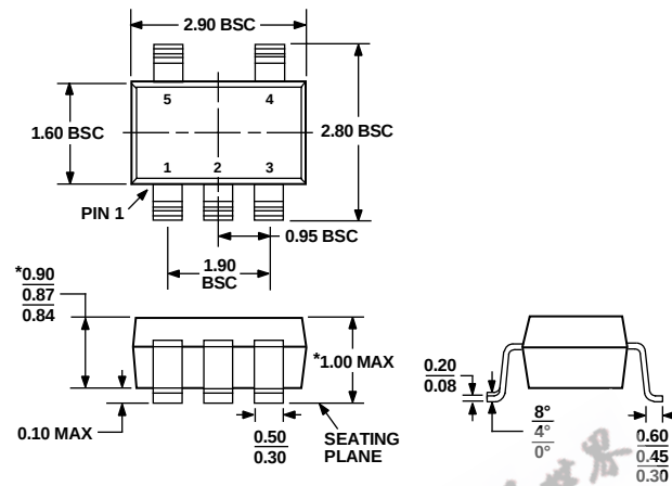
Figure 30. 5-Lead Thin Small Outline Transistor Package [TSOT] (UJ-5)
