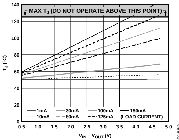
Figure 26. 500 mm 2 of PCB Copper, T_A = 50^\circ\text{C}
