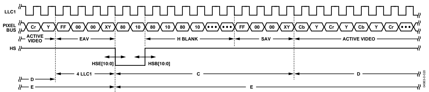
Figure 20. HS Timing
