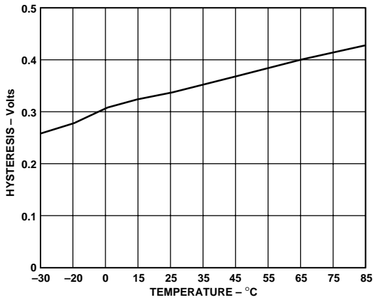
Figure 1. Hysteresis vs. Temperature for SU1—Low to High
