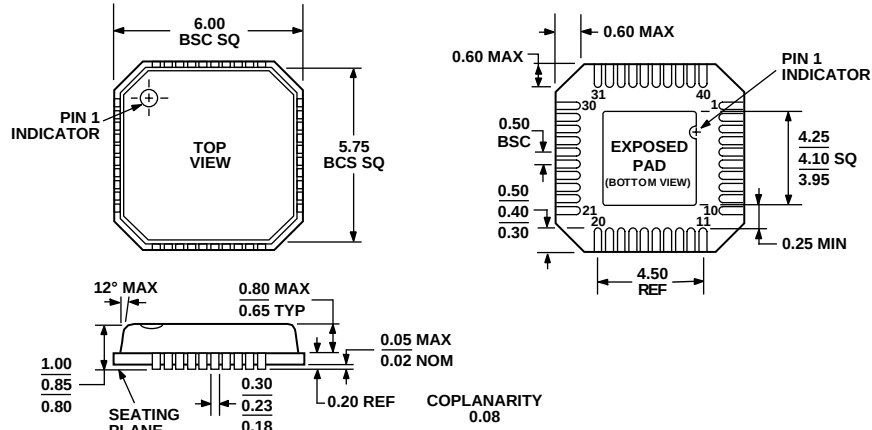
COMPLIANT TO JEDEC STANDARDS MO-220-VJJD-2 Figure 43. 40-Lead Lead Frame Chip Scale Package [LFCSP] (CP-40) Dimensions shown in millimeters
