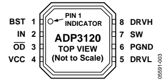
Figure 3. 8-Lead LFCSP Pin Configuration
