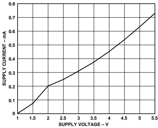
Figure 2. Power Supply Current vs. Voltage
