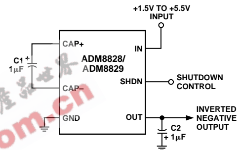
Figure 12. Typical Circuit Configuration
