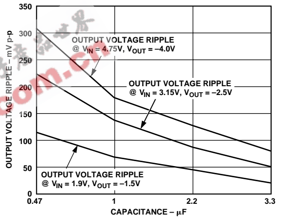
Figure 6. Output Voltage Ripple vs. Capacitance
