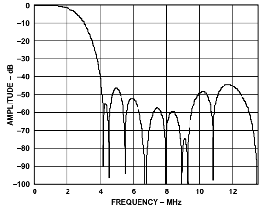
Figure 11. PAL UV Filter
