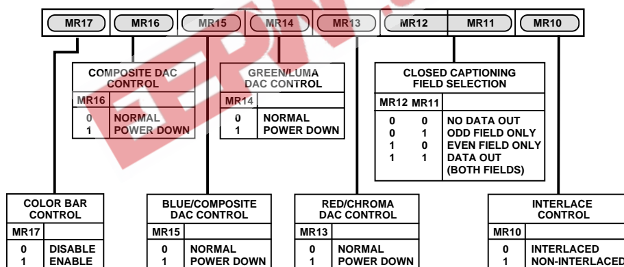
Figure 32. Mode Register 1
