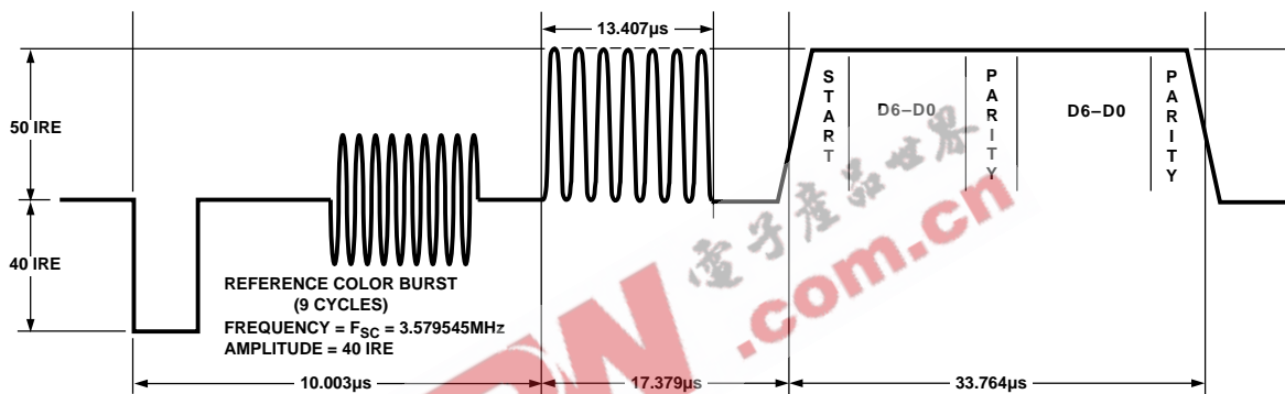
Figure 43. Closed Captioning Waveform (NTSC)
