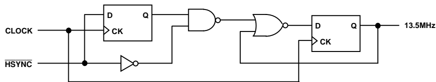
Figure 42. Circuit to Generate 13.5 MHz
