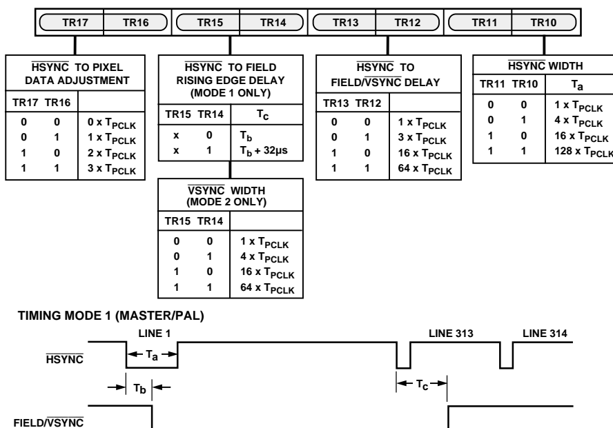
Figure 37. Timing Register 1
