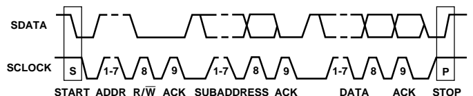
Figure 28. Bus Data Transfer
