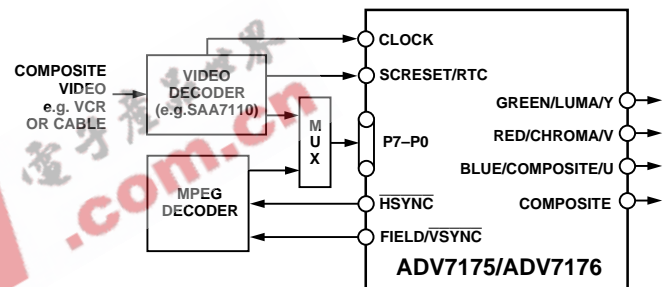
Figure 12. RTC Connections
