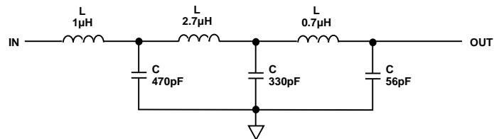
Figure 56. Output Filter
