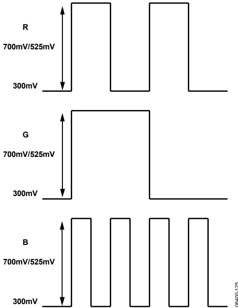
Figure 124. SD/ED RGB Output Levels—RGB Sync Disabled
