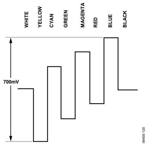
Figure 119. Pb Levels—PAL
