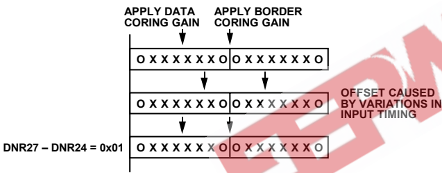
Figure 78. SD DNR Offset Control
