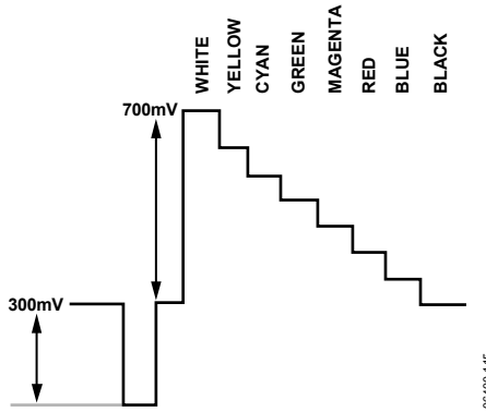
Figure 114. Y Levels—NTSC
