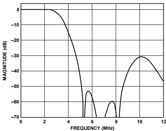
Figure 42. SD Chroma 2.0 MHz Low-Pass Filter Response
