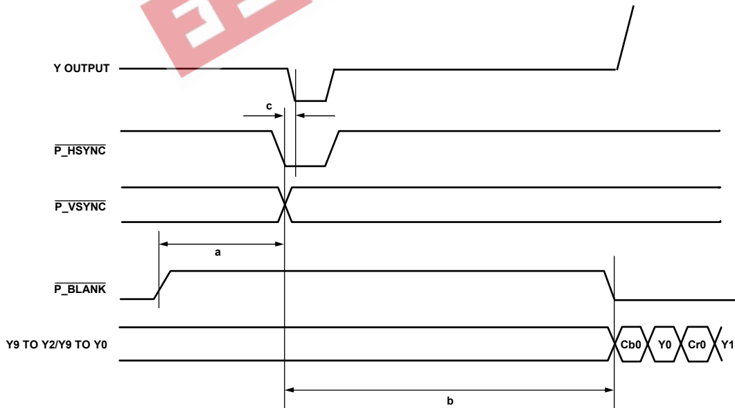
Figure 14. ED-SDR, 16-/20-Bit, 4:2:2 YCrCb ( \overline{\text{HSYNC}} / \overline{\text{VSYNC}} ) Input Timing Diagram
