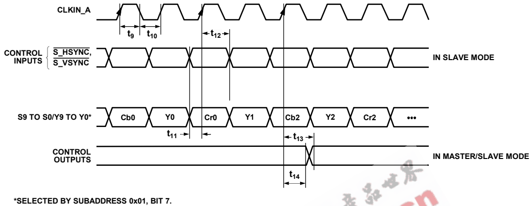
Figure 2. SD Only, 8-/10-Bit, 4:2:2 YCrCb Pixel Input Mode (Input Mode 000)
