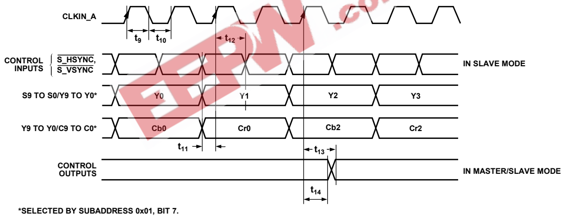
Figure 3. SD Only, 16-/20-Bit, 4:2:2 YCrCb Pixel Input Mode (Input Mode 000)
