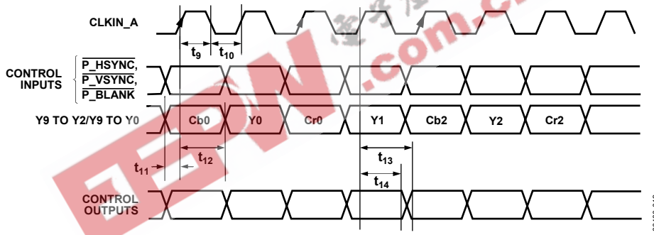
Figure 12. ED Only (at 54 MHz), 8-/10-Bit, 4:2:2 YCrCb (HSYNC/VSYNC) Pixel Input Mode (Input Mode 111)
