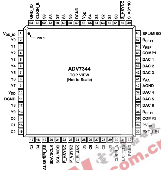
Figure 21. Pin Configuration
