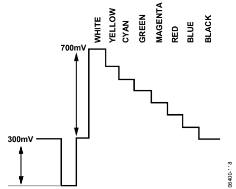
Figure 117. Y Levels—PAL
