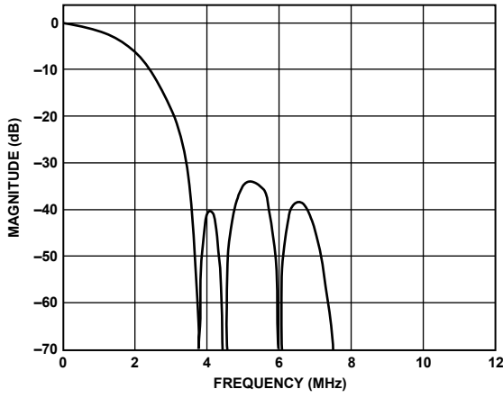
Figure 40. SD Luma QCIF Low-Pass Filter Response
