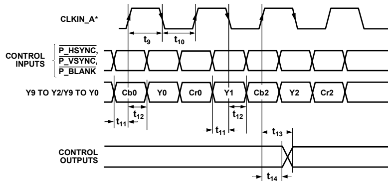
Figure 8. ED/HDD-DDR Only, 8-/10-Bit, 4:2:2 YCrCb (HSYNC/VSYNC) Pixel Input Mode (Input Mode 010)
