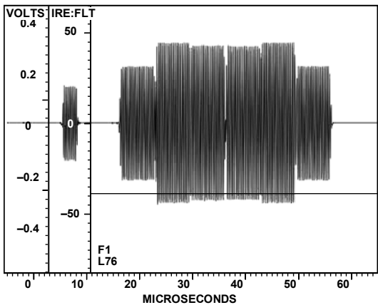
Figure 130. NTSC Chroma
