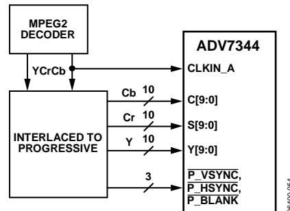
Figure 54. ED/HD Only Example Application
