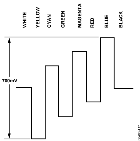
Figure 116. Pb Levels—NTSC
