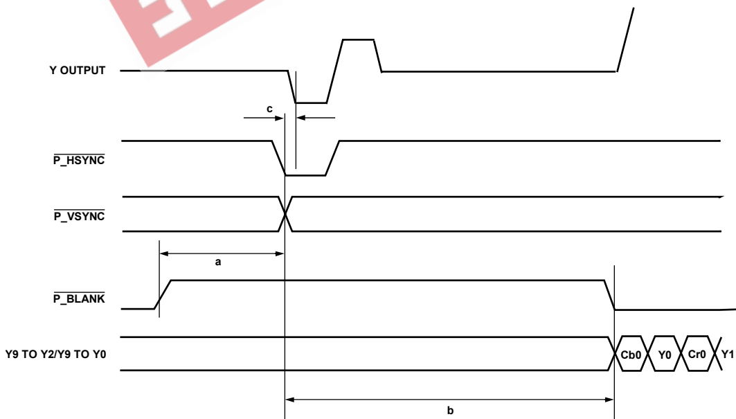
Figure 16. HD-SDR, 16-/20-Bit, 4:2:2 YCrCb ( \overline{\text{HSYNC}} / \overline{\text{VSYNC}} ) Input Timing Diagram
