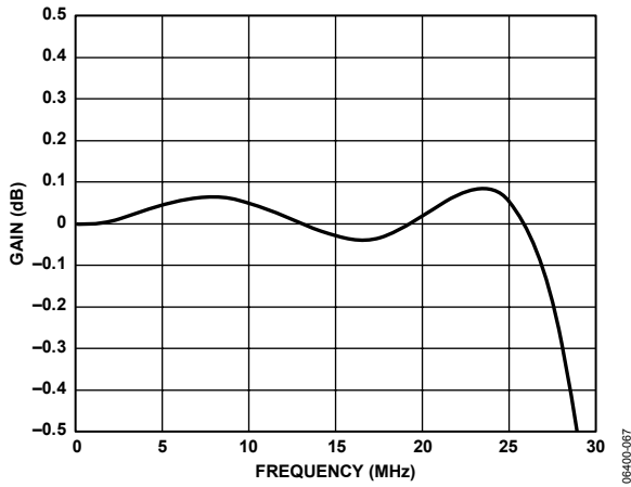
Figure 66. ED/HD Sinc Compensation Filter Enabled
