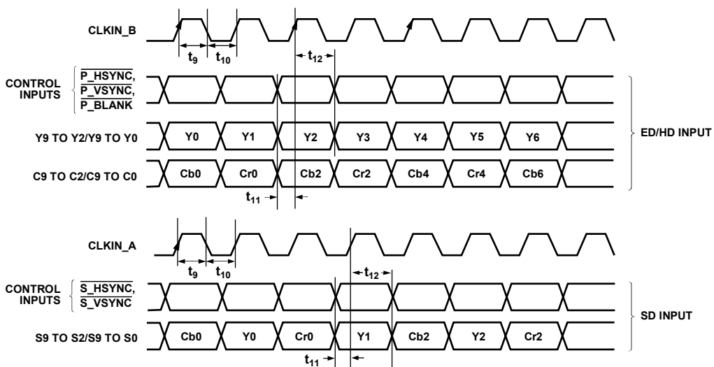
Figure 10. SD, ED/HDD-SDR Input Mode, 16-/20-Bit, 4:2:2 ED/HDD and 8-/10-Bit, SD Pixel Input Mode (Input Mode 011)
