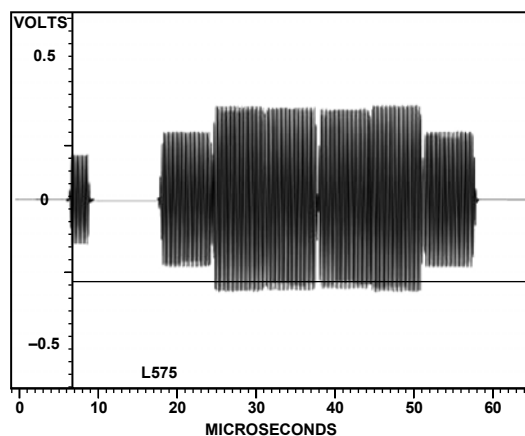
Figure 132. PAL Luma
