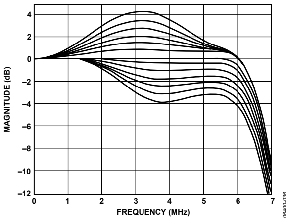
Figure 36. SD Luma SSAF Filter, Programmable Responses
