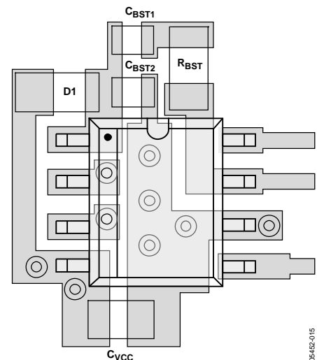
Figure 14. External Component Placement Example
