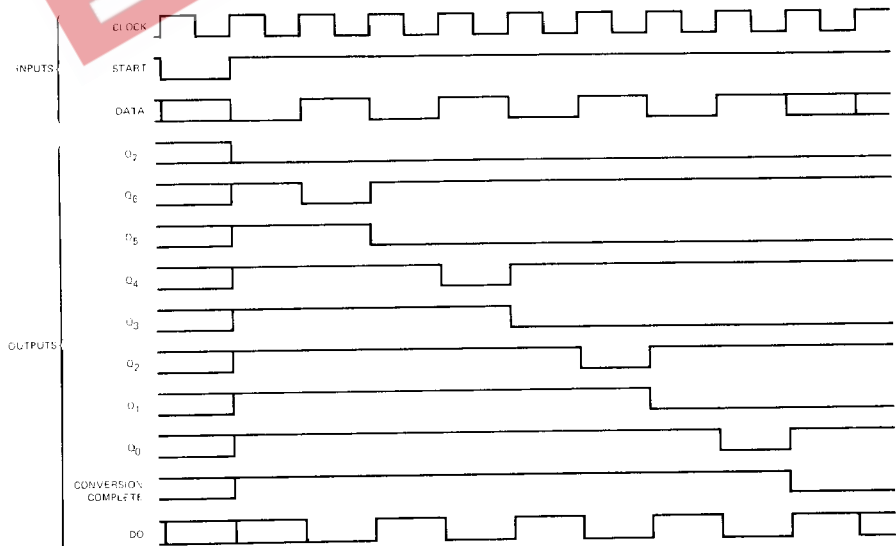
Am25(L)02/3 TIMING CHART
