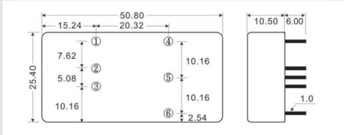
MECHANICAL DIMENSION (Top View)
