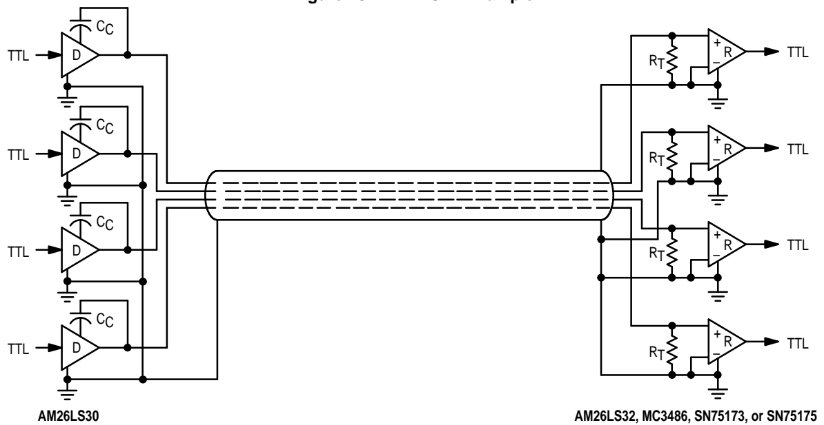
Figure 18. EIA-423-A Example
