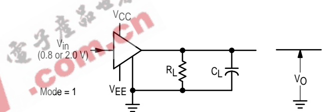
Figure 2. Single-Ended Output Test
