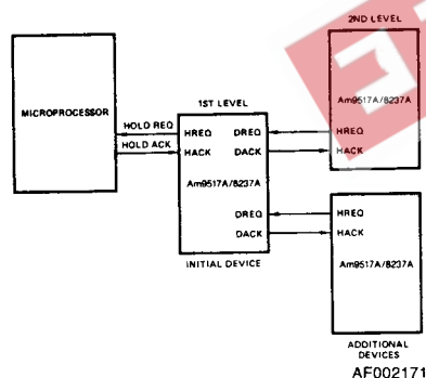
Figure 1. Cascaded Am9517A/8237As
