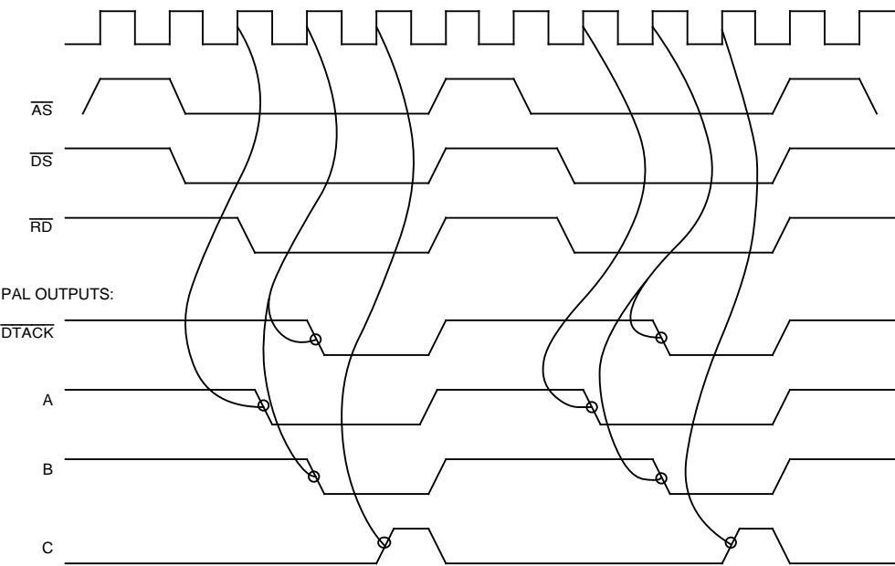
Figure 7–15. PAL Timing
