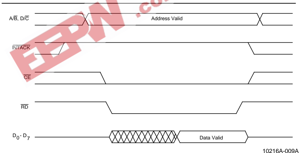
Figure 2–1. SCC Read Cycle
