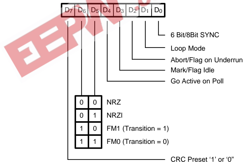
Figure 6–11. Write Register 10
