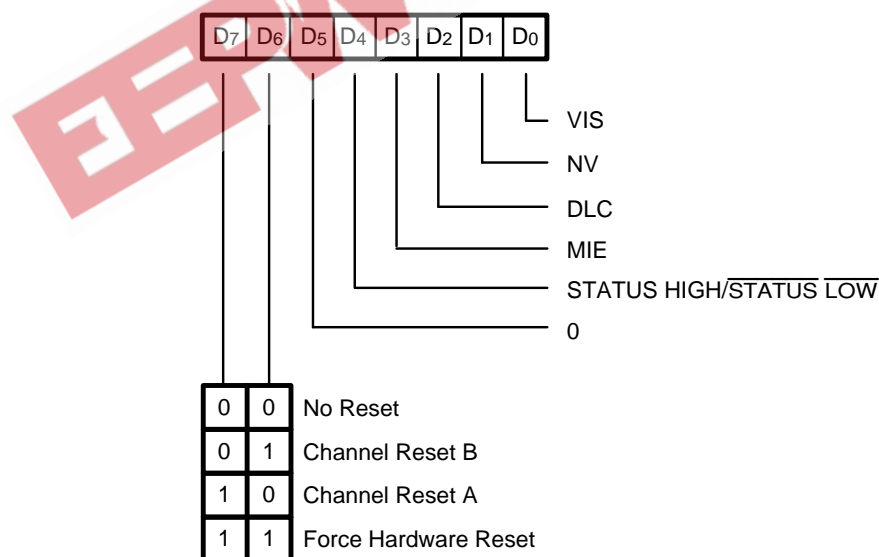
Figure 7–1. Write Register 9
