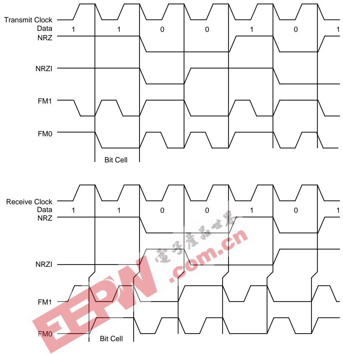
Figure 6–12. NRZ (NRZI) FM1 (FM0) Timing
