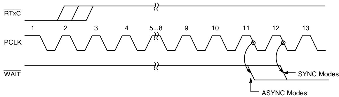
Figure 3–10. \overline{\text{DTR/REQ}} Activation
