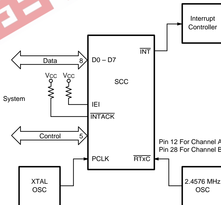
Figure 7-4. SCC Interface
