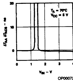
Access Time Change Versus Input Voltage
