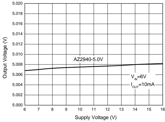
Figure 4. Line Regulation
