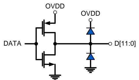
FIGURE 46. CMOS OUTPUTS
