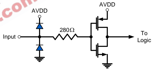
FIGURE 44. DIGITAL INPUTS
