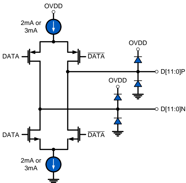
FIGURE 45. LVDS OUTPUTS
