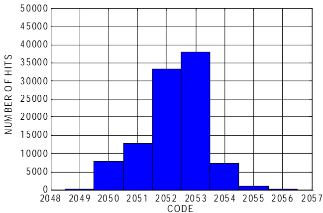
FIGURE 14. NOISE HISTOGRAM
