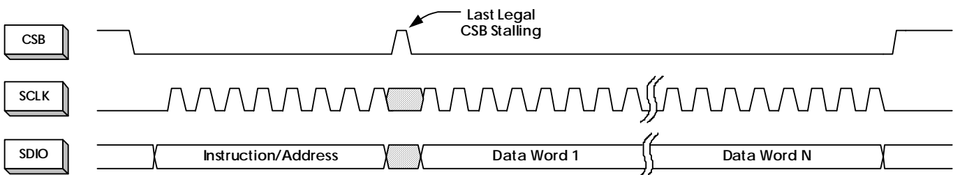
FIGURE 37. N-BYTE TRANSFER
