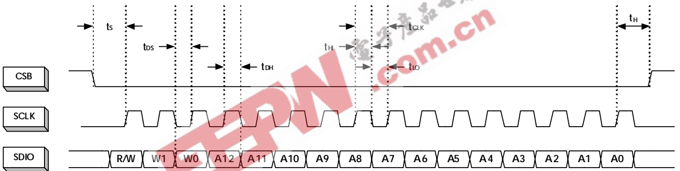
FIGURE 35. INSTRUCTION/ADDRESS PHASE
