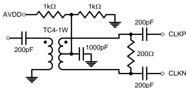
FIGURE 29. RECOMMENDED CLOCK DRIVE
