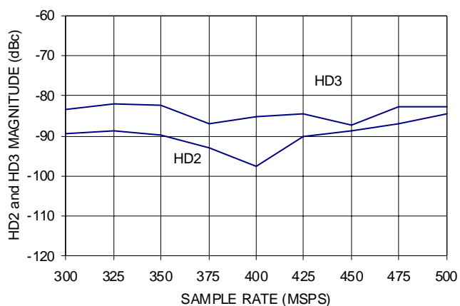
FIGURE 9. HD2 AND HD3 vs f SAMPLE
