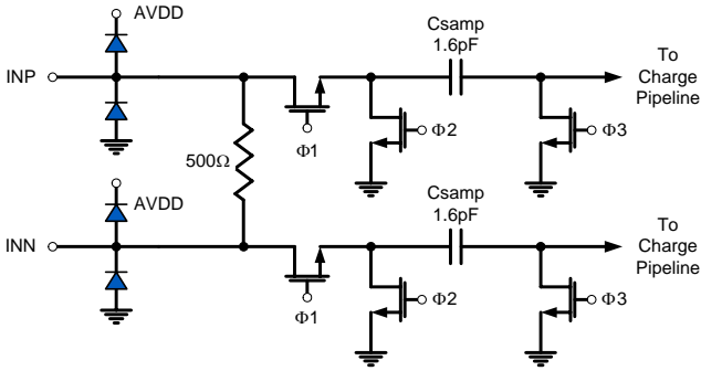
FIGURE 41. ANALOG INPUTS
