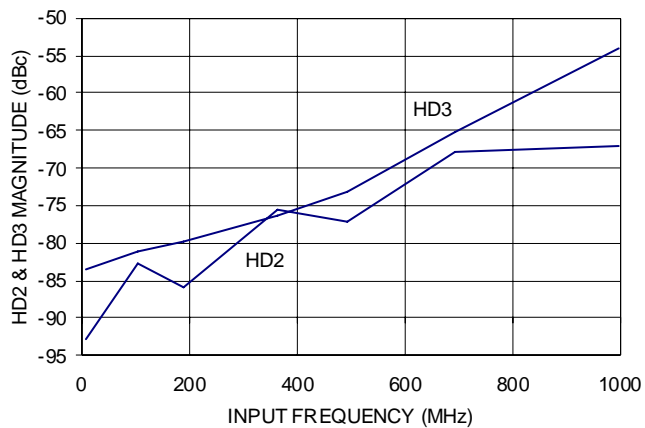
FIGURE 5. HD2 AND HD3 vs f IN
