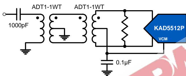
FIGURE 26. TRANSFORMER INPUT FOR GENERAL PURPOSE APPLICATIONS
