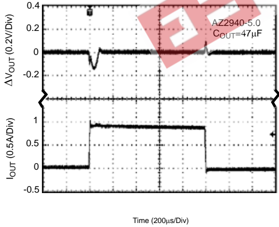
Figure 18. Load Transient
