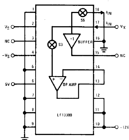
Test Circuit 4 -VB Voltage Measurement Test
