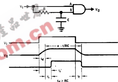
FIGURE 7. Rise Time Delay Circuit
