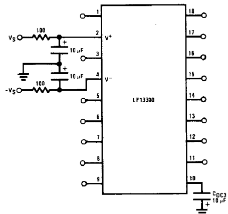
FIGURE 9. Power Supply Noise Reduction Circuit
