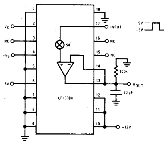
Test Circuit 6 Op Amp Slew Rate Test
