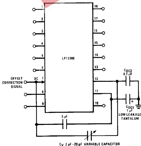
FIGURE 8. Residual Offset Nulling Circuit
