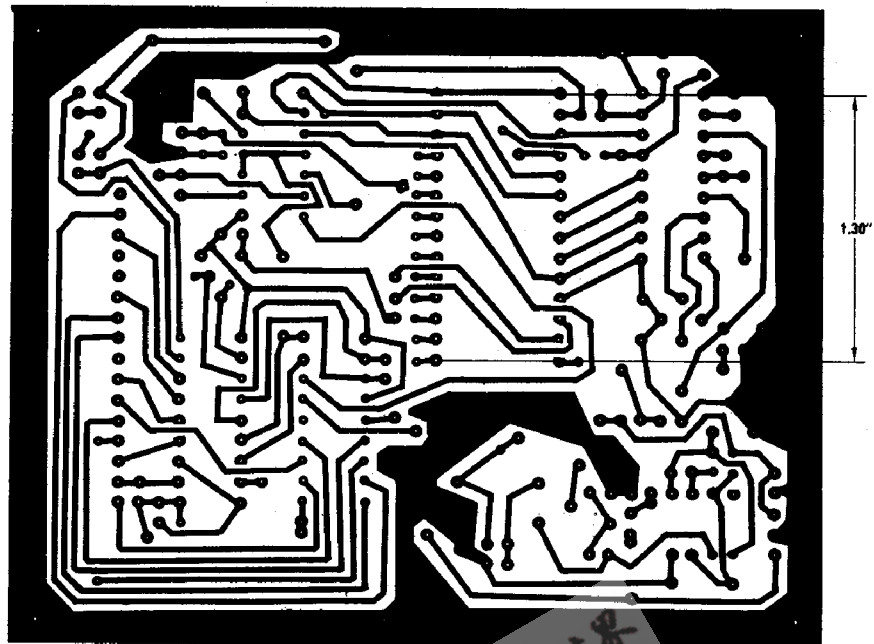
FIGURE 16. PC Board for 3 3/4 Plus (±8191 Counts) and 3 1/2-Digit DPM
