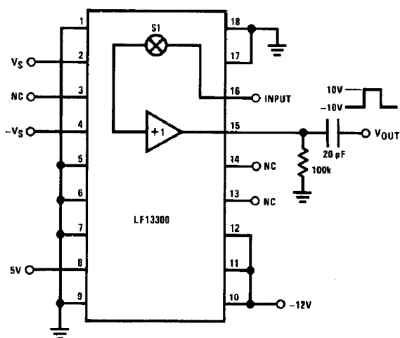
Test Circuit 9 Buffer Slew Rate Test
