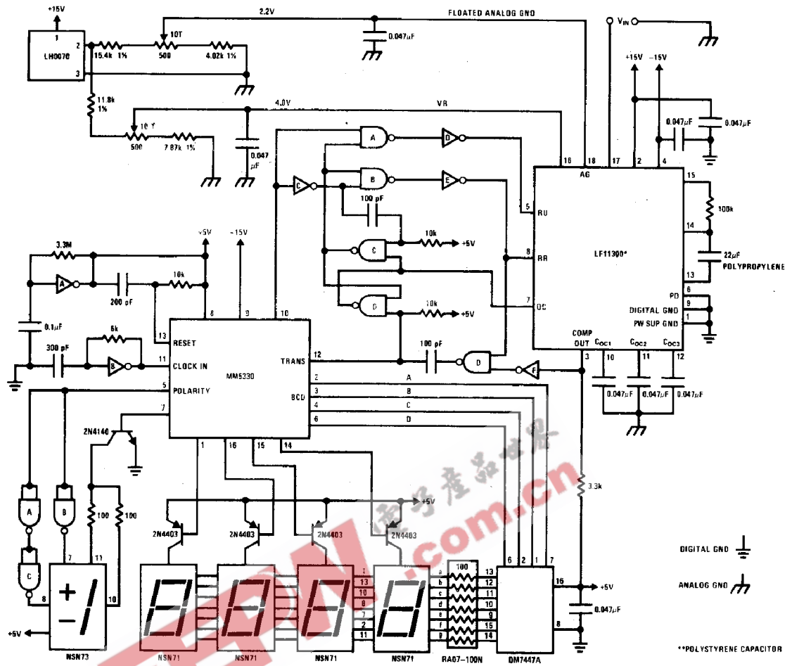
FIGURE 18. LF11300, MM5330 DPM Application
