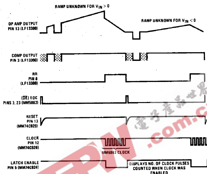
FIGURE 15. Timing Diagram for 3 3/4-Digit DVM
