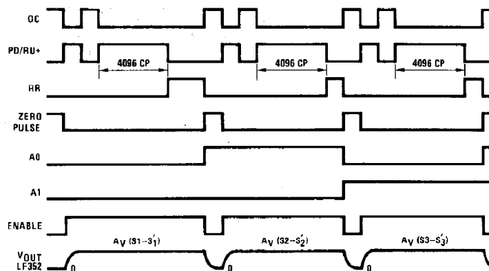
FIGURE 13. Timing Diagram for Figure 12
