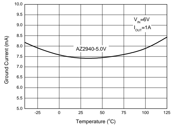
Figure 11. Ground Current vs. Temperature
