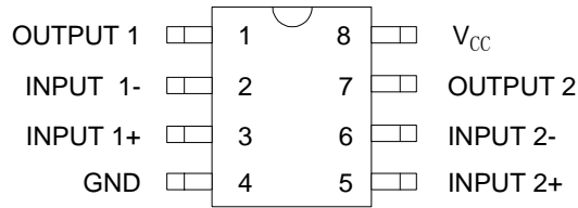
Figure 2. Pin Configuration of AZ358/358C (Top View)
