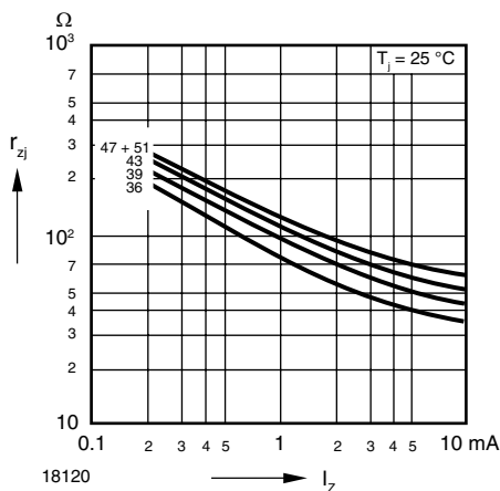
Figure 3. Dynamic Resistance vs. Zener Current
