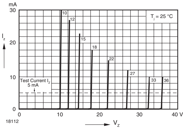
Figure 13. Breakdown Characteristics
