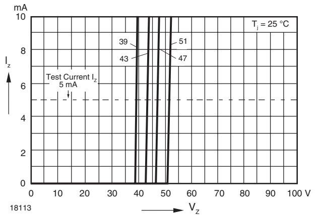
Figure 14. Breakdown Characteristics
