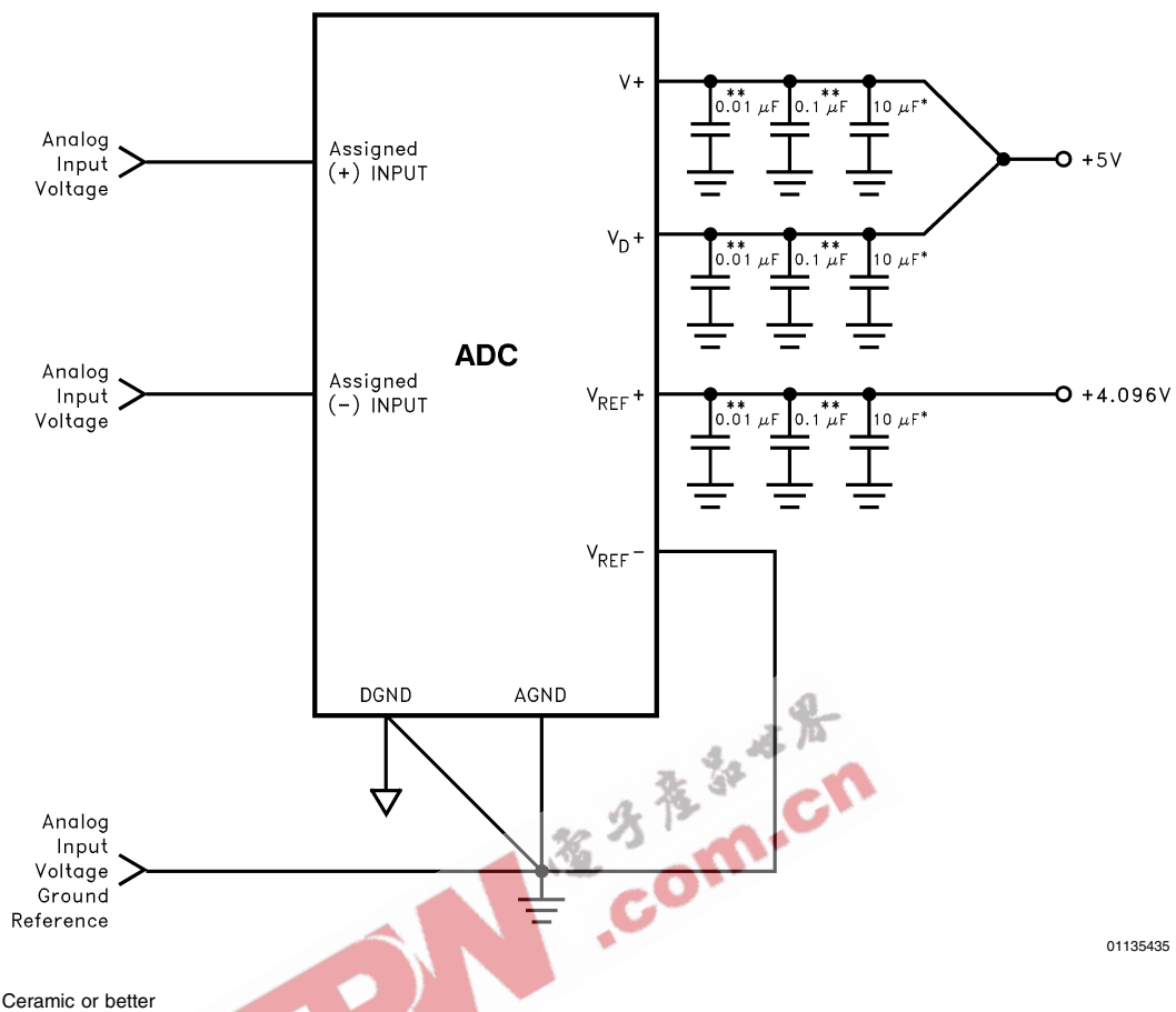
FIGURE 6. Recommended Power Supply Bypassing and Grounding
