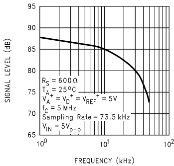
Bipolar Spurious Free Dynamic Range
