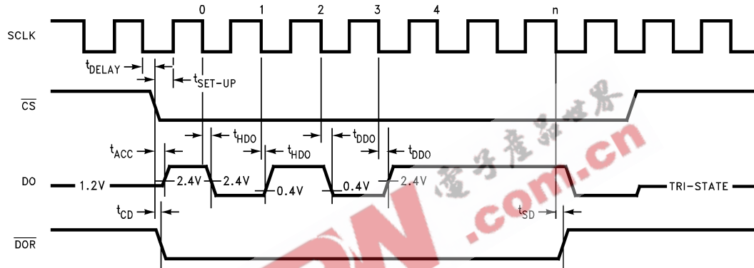
DO Data Output Timing Using \overline{\text{CS}}
