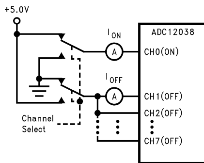
Leakage Current
