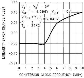
Linearity Error Change vs Clock Frequency
