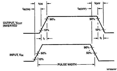
Figure 2 Switching Waveforms
