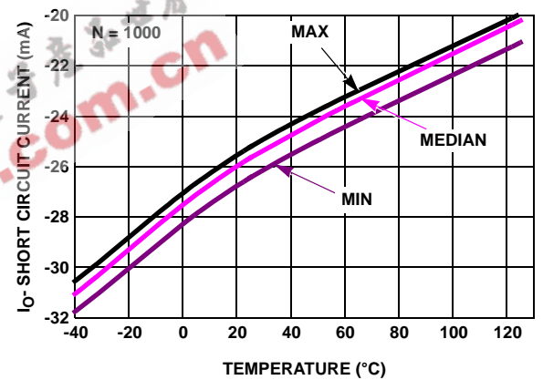
FIGURE 40. I_{O-} SHORT CIRCUIT OUTPUT CURRENT vs TEMPERATURE, V_{IN} = +2.55V , R_L = 10k , V_+ = 5V , V_- = 0V
