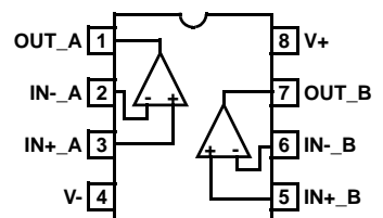
ISL28268 (8 LD MSOP) TOP VIEW
