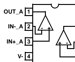
ISL28268 (8 LD SOIC) TOP VIEW
