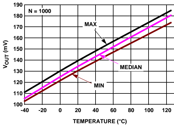
FIGURE 37. V_{OUT} LOW vs TEMPERATURE, V_+ = 5V , V_- = 0V , V_{CM} = 2.5V , R_L = 1k
