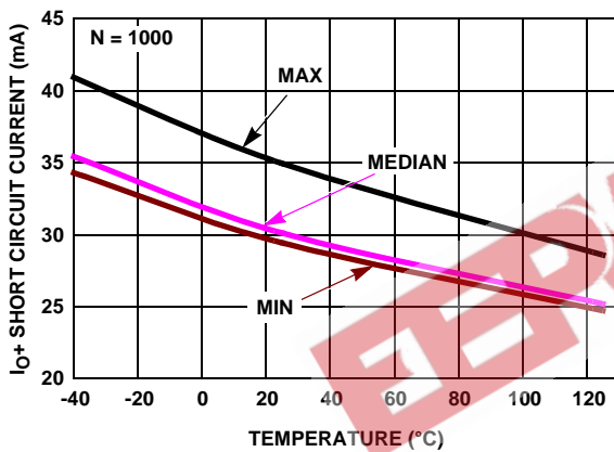
FIGURE 39. I_{O+} SHORT CIRCUIT OUTPUT CURRENT vs TEMPERATURE, V_{IN} = -2.55V , R_L = 10k , V_+ = 5V , V_- = 0V
