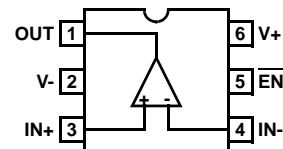
ISL28168 (6 LD SOT-23) TOP VIEW
