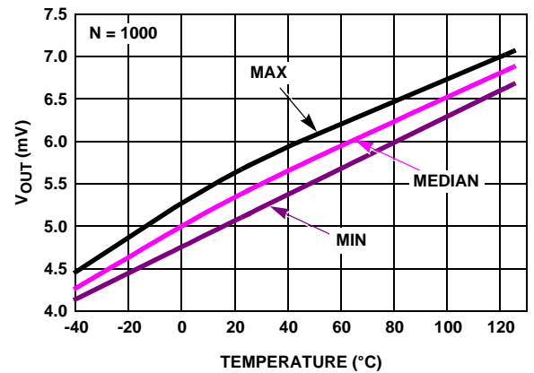
FIGURE 38. V_{OUT} LOW vs TEMPERATURE, V_+ = 5V , V_- = 0V , V_{CM} = 2.5V , R_L = 100k
