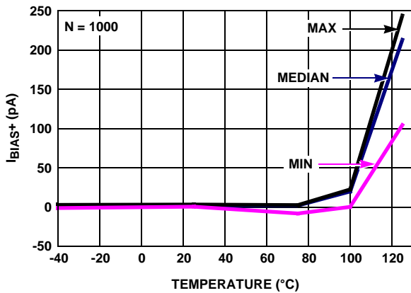
FIGURE 25. I_{BIAS+} vs TEMPERATURE, V_+ , V_- = \pm 2.5V
