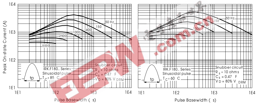
Fig. 11 - Frequency Characteristics
