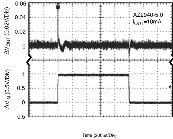
Figure 19. Line Transient
