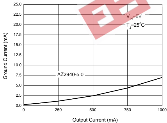
Figure 6. Ground Current vs. Output Current
